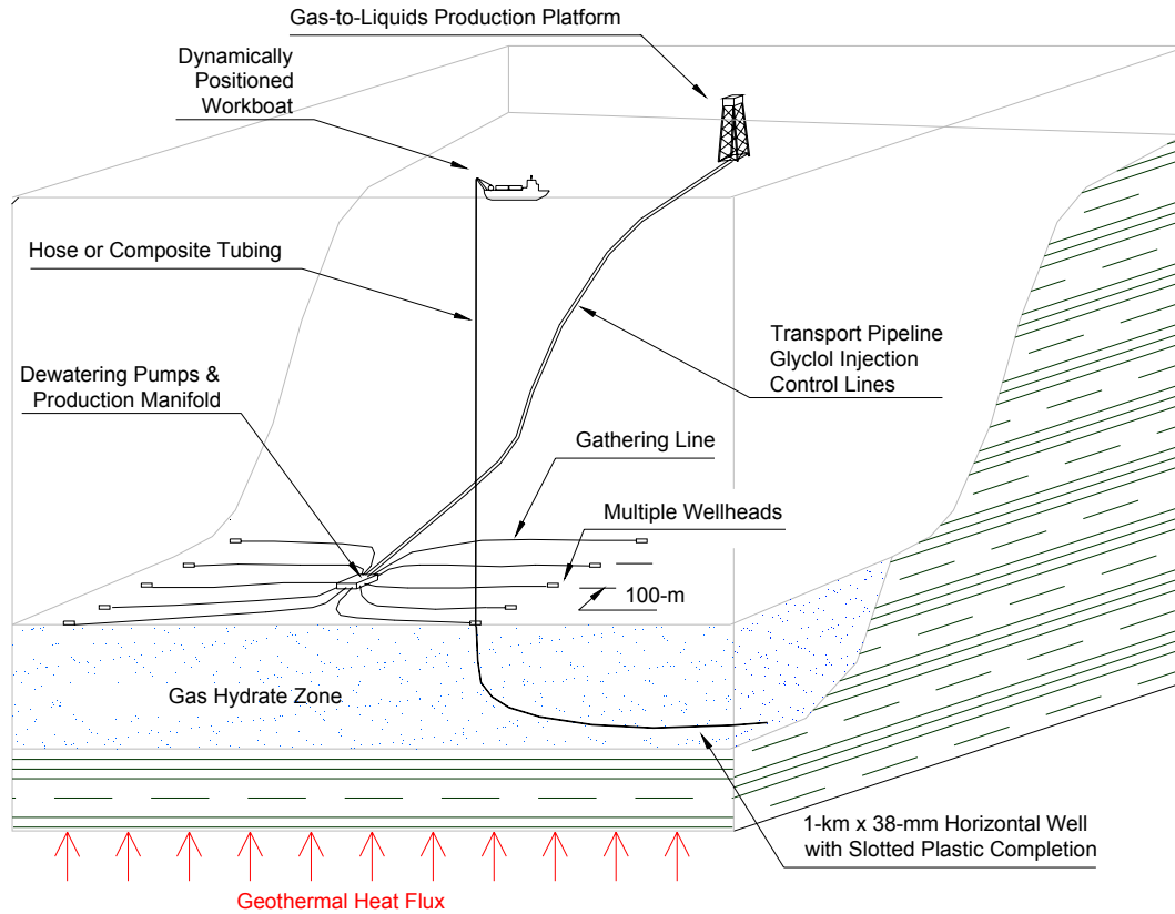
Figure 3. Riserless drilling and production system for gas hydrates.
