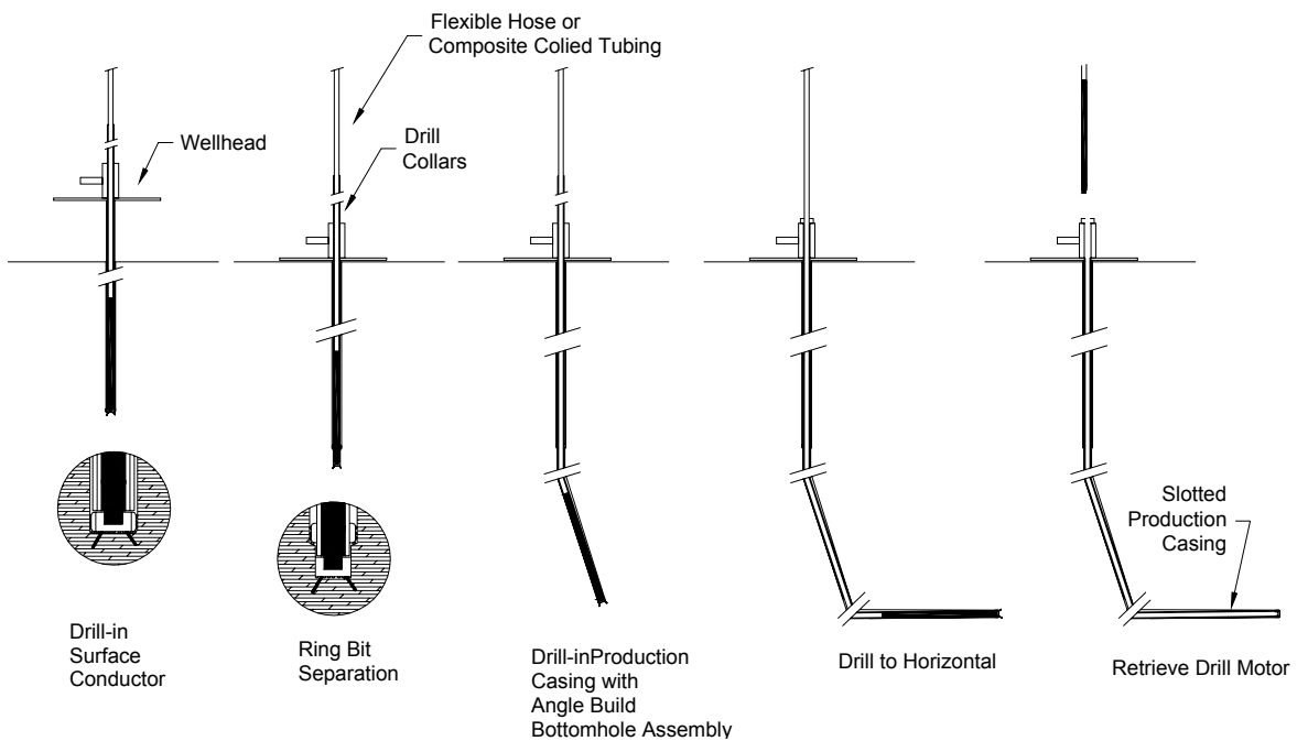
Figure 4. Detail of horizontal well placement using drill-in casing techniques with coiled tubing.
